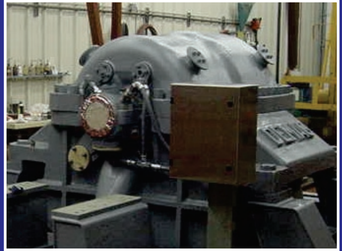
Demag KA10 Oxygen Compressor
