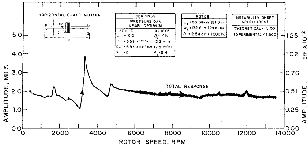
Figure 15. Total response, near optimum pressure dam bearings.
