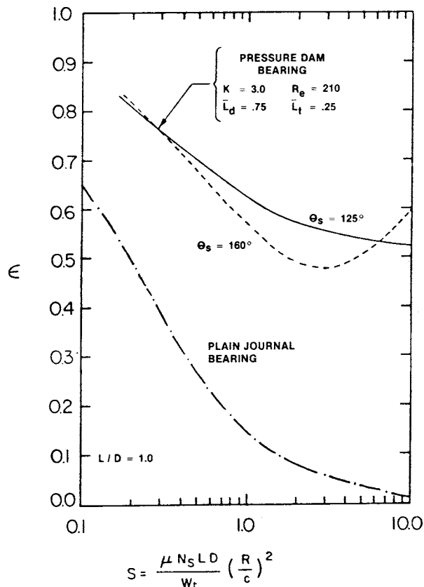
Figure 9. Pressure dam and plain journal bearing eccentricity ratios.
