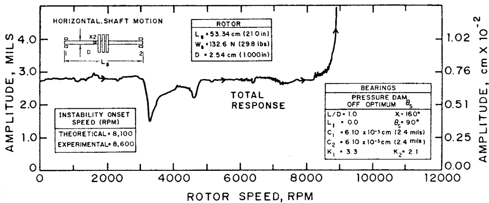
Figure 19. Total response, off-optimum step location, pressure dam bearings.
