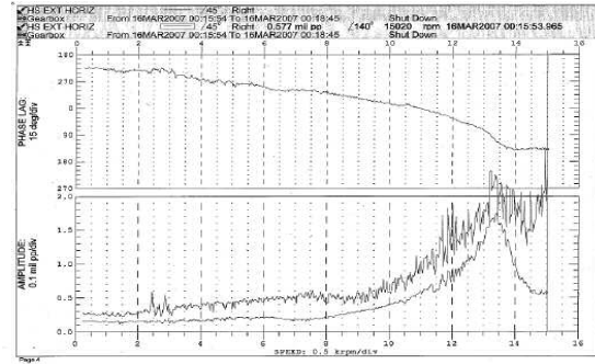
Figure 4. Initial Pinion Response, Q = 34 gpm, C_b = 9.0 mils, Fabricated Baseplate.
