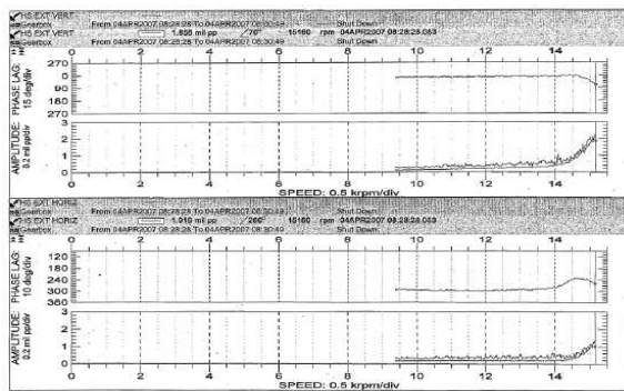
Figure 6. Interim Pinion Response, P_{in} = 45 psi, Q = 60 gpm, C_b = 9.0 mils, Solid Baseplate.
