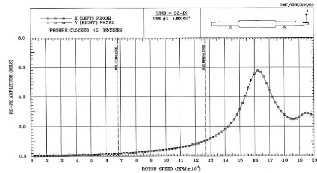
Figure 21. Predicted Pinion Response, Starvation Model with K = 70 Percent and C = 15 Percent of Full Film Values, C_b = 9.0 mils, K_s = 20.0 \times 10^6 lbf/in, with Integral Flange.
