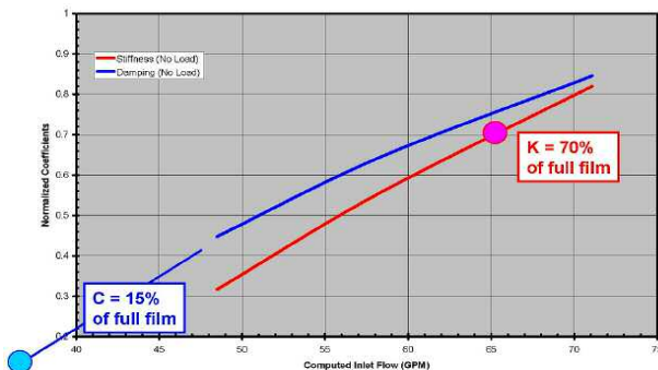
Figure 14. Starvation Model, Normalized K and C Versus Oil Flow Showing K = 70 Percent and C = 15 Percent of Full Film Values.
