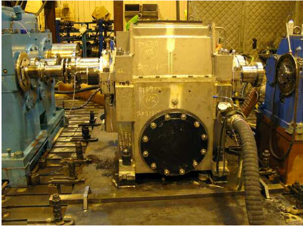
Figure 2. Problem Gearbox During Mechanical Testing.
