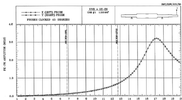
Figure 11. Predicted Pinion Response, Full Film, C_b = 9.0 mils, K_s = 20.0 \times 10^6 lbf/in.
