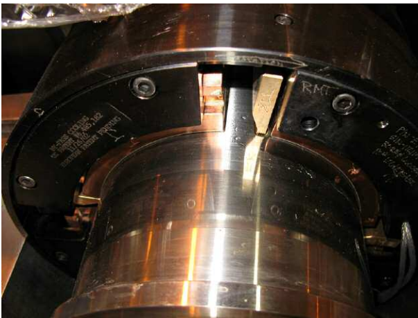
Figure 3. Tilting Pad Journal Pinion Bearing—Evacuated Housing Design.
