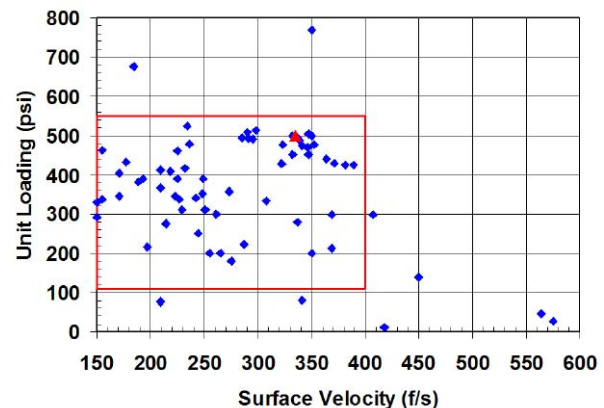
Figure 1. Tilting Pad Journal Bearing Severe Application Experience Plot.
