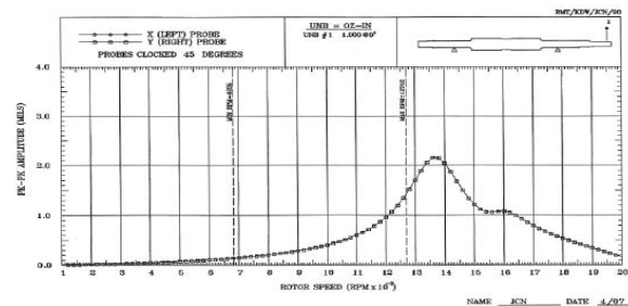
Figure 8. Predicted Pinion Response, Full Film, C_b = 9.0 mils, K_s = 7.0 \times 10^6 lb/in.
