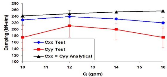
Figure 16. 4x4 Inch TPJB Zero Load Test Data—Principal Damping Versus Oil Flow.
