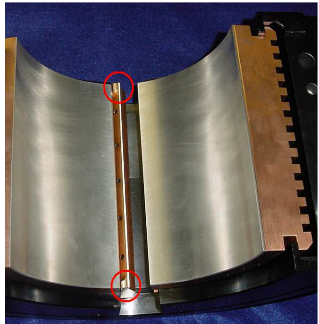
Figure 19. Spray-bar blocker Side Shields Protecting the Inlet Oil.
