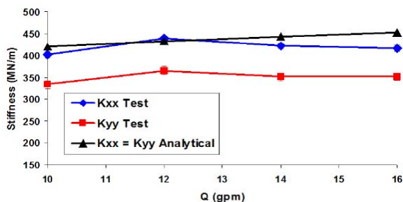
Figure 15. 4x4 Inch TPJB Zero Load Test Data—Principal Stiffness Versus Oil Flow.
