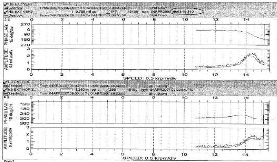
Figure 5. Interim Pinion Response, P_{in} = 25 psi, Q = 45 gpm, C_b = 9.0 mils, Solid Baseplate.
