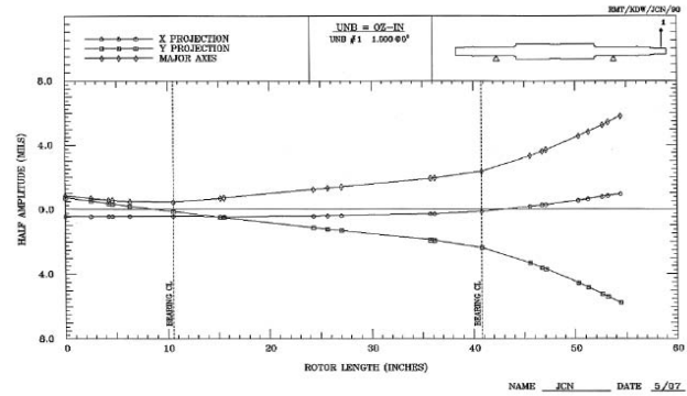
Figure 20. Pinion Mode Shape with Coupling Hub Attachment.
