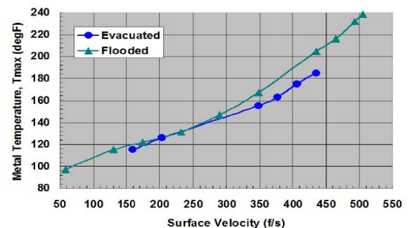
Figure 18. Evacuated Versus Flooded TPJB, High Speed Balance on Laminations.
