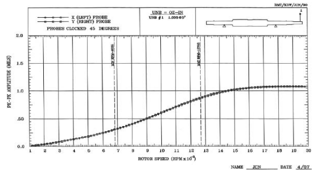
Figure 12. Predicted Pinion Response, Starvation Model with 52 Degree Pad Arc Length, 50 Percent Pad Pivot Offset, C_b = 9.0 mils, K_s = 20.0 \times 10^6 lbf/in.
