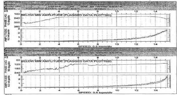
Figure 7. Final Pinion Response, Q = 55 gpm, C_b = 7.5 mils, Solid Baseplate.
