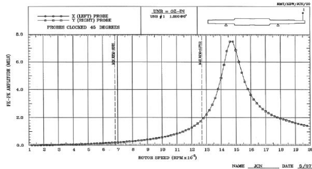
Figure 13. Predicted Pinion Response, Starvation Model with K = 70 Percent and C = 15 Percent of Full Film Values, C_b = 9.0 mils, K_s = 20.0 \times 10^6 lbf/in.
