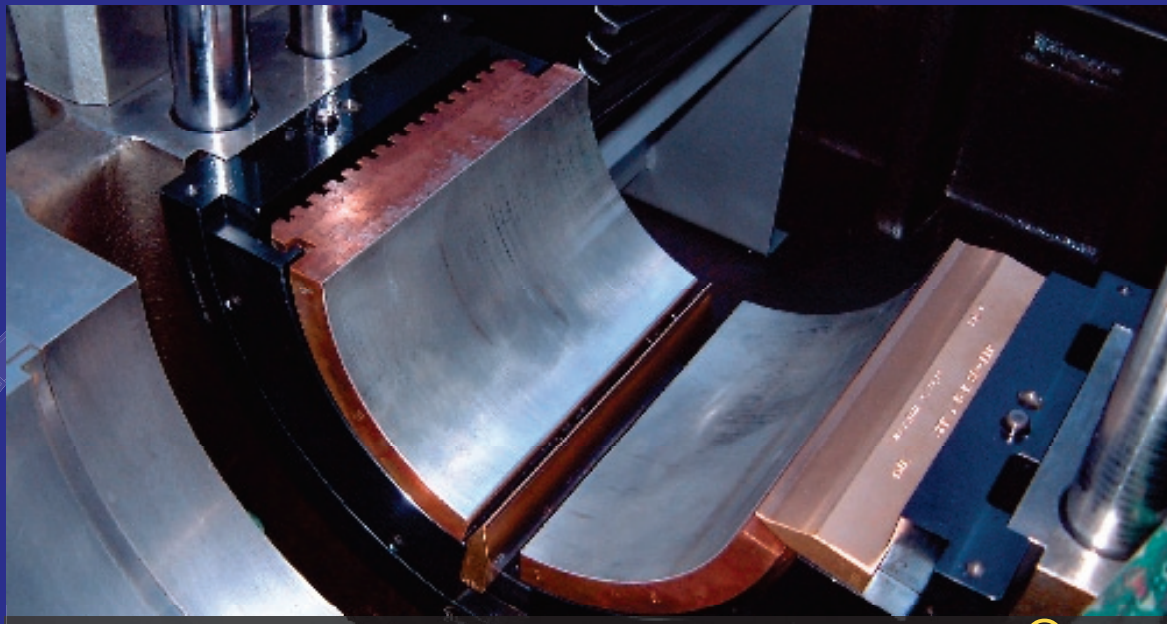
7.8" High Speed Pinion RMT Ultra-Bearing® with Spray-Bar Blockers® and By-Pass Cooling®
